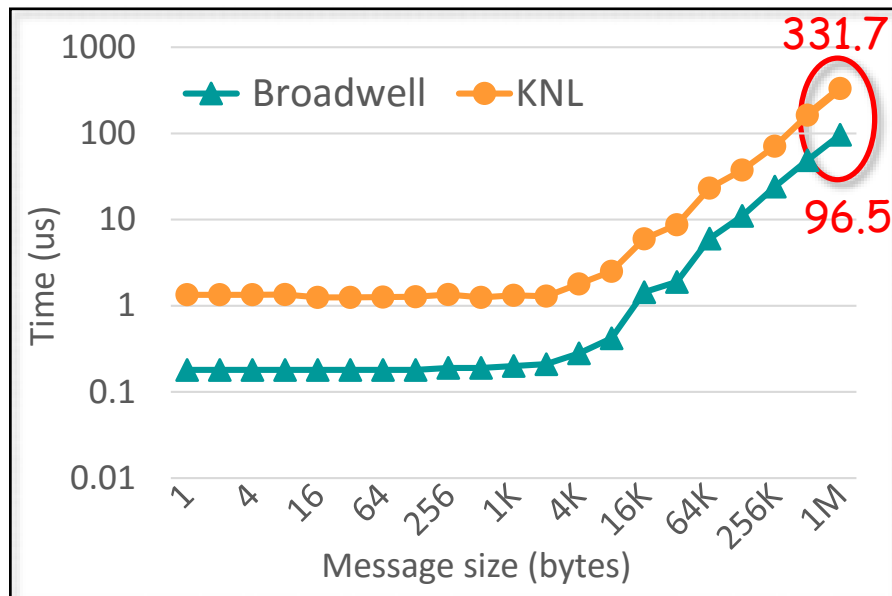
Shmem_putmem
