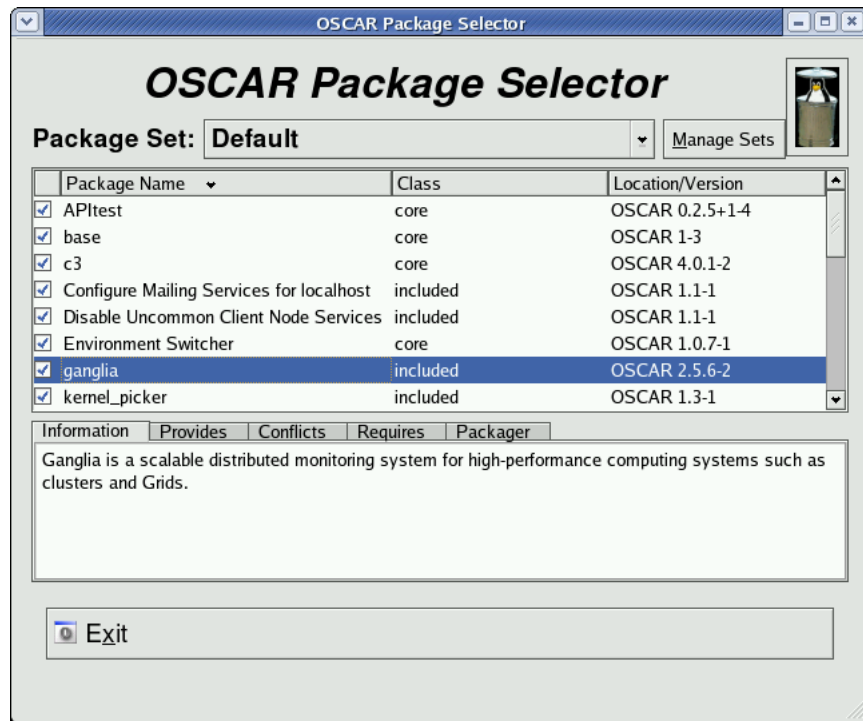
Figure 17: Selecting which OSCAR packages to install.
