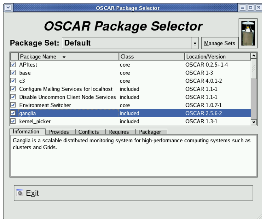
Figure 2: OSCAR package selection.
