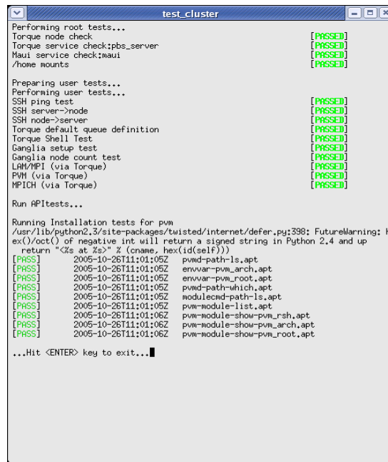
Figure 34: Test the cluster.
