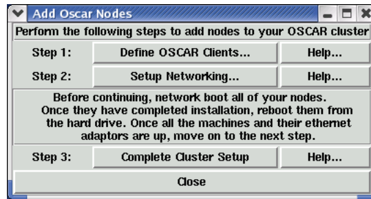
Figure 36: Add OSCAR Clients.
