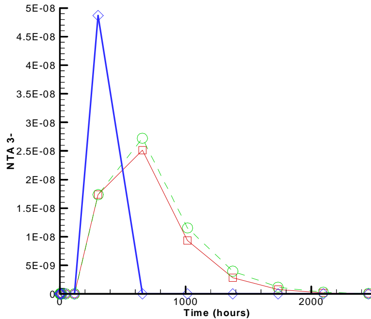
Figure 6.12. Total aqueous (a) \text{Co}^{2+} and (b) \text{NTA}^{3-} at the extraction well over time when subjected to flushing of adsorbed species ( F / dashed line) versus flushing plus biodegradation ( G / solid line). A nonreactive tracer is plotted ( \diamond / bold line) for comparison.
