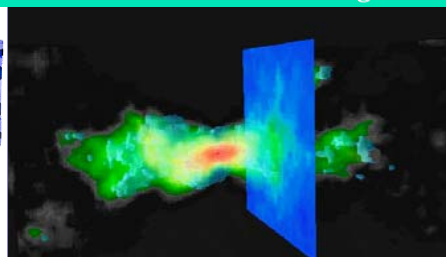
Lattice quantum chromodynamics
