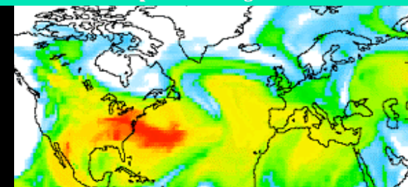
Perturbation in clear-sky and cloud albedo
