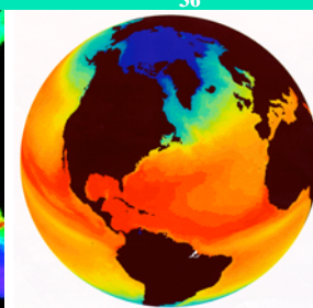
Sea surface temperature
