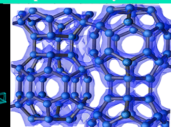
Crystal structure for C_{36} solid
