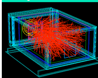
Au-Au collision
