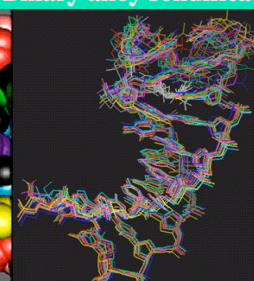
Structural biology
