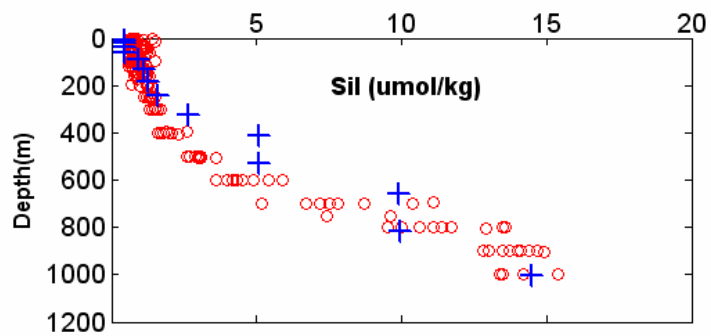
Bermuda Station (31° 40' N; 64° 10' W): Monthly climatology (January), model (blue), observations (red)
